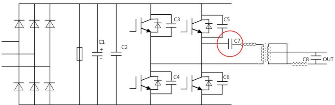
C7:谐振选频电容 The resonant frequency capacitor
